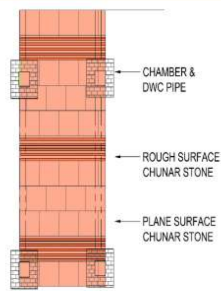
PLAN OF CHUNAR STONE ROAD WORK (75 % PLANE & 25 % OF ROUGH SURFACE)
